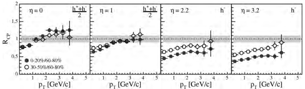
FIGURE 11. R_{cp} for central (full points) and semi-central (open points) d+^{197}\text{Au} collisions as a function of pseudo-rapidity.
