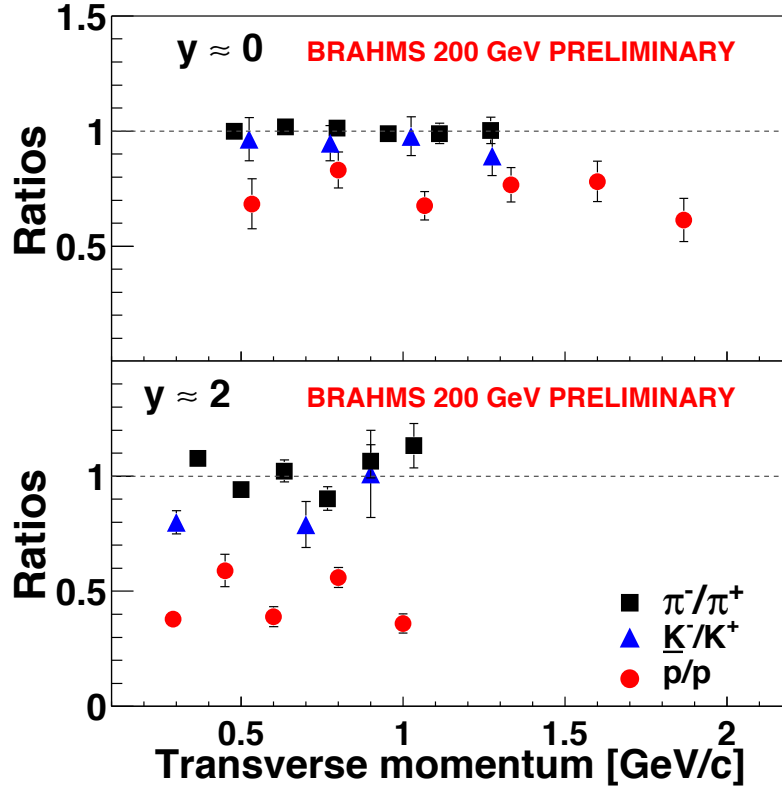
Fig. 12. Anti-particle particle ratios versus p_t , for y \approx 0 (top panel) and y \approx 2 (bottom panel) (see text for more details).
