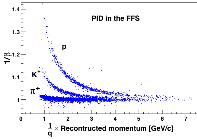
Fig. 9. Particle identification in the FFS.
