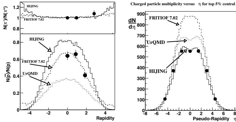
Fig. 15. Comparison of the measured N(\bar{p})/N(p) (lower panel) and N(\pi^-)/N(\pi^+) (upper panel) ratios to model predictions. The data shown are for 0 – 40% central events and integrated over the transverse momentum range shown in Fig. 11. The three model calculations (HIJING, FRITIOF, and UrQMD) are shown for comparison. See text for details.
