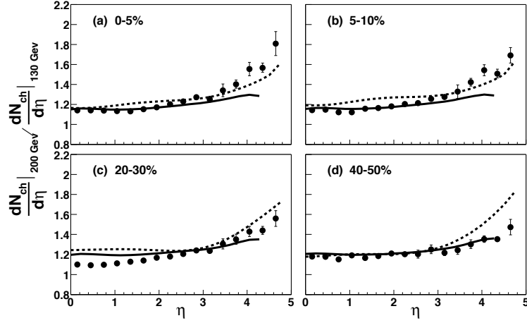
Fig. 6. Ratio of dN_{ch}/d\eta values at \sqrt{s_{NN}}=200 GeV and 130 GeV compared to the model calculations (see Fig. 3 caption). Total uncertainties are shown, assuming a 3% relative scaling uncertainty between the two energies.
