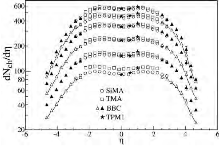
Fig. 3. Distributions of dN_{ch}/d\eta for centrality ranges of, top to bottom, 0-5%, 5-10%, 10-20%, 20-30%, 30-40%, and 40-50%. Statistical uncertainties are shown where larger than the symbol size. The connecting lines and alternating open and closed symbols for the BBC data are to help distinguish points associated with different centrality ranges.
