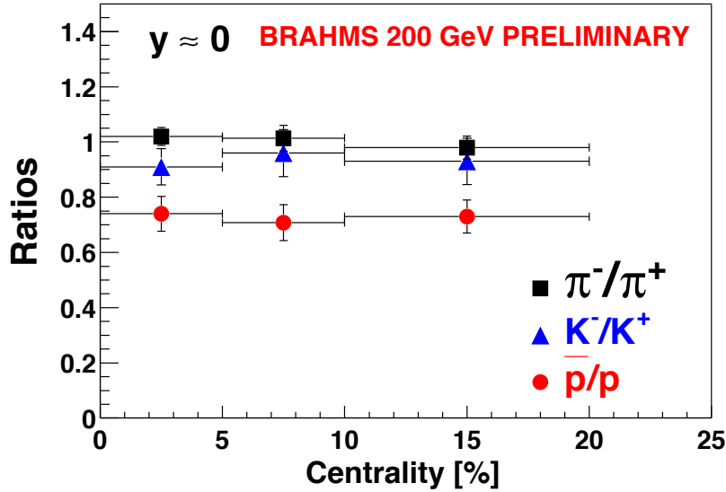
Fig. 13. Anti-particle to particle ratios versus collision centrality.
