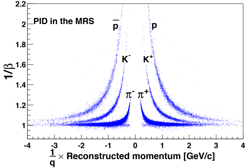
Fig. 8. Particle identification in the MRS.
