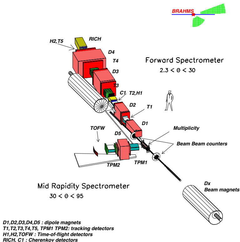
Fig. 1. The BRAHMS experiment setup in perspective.
