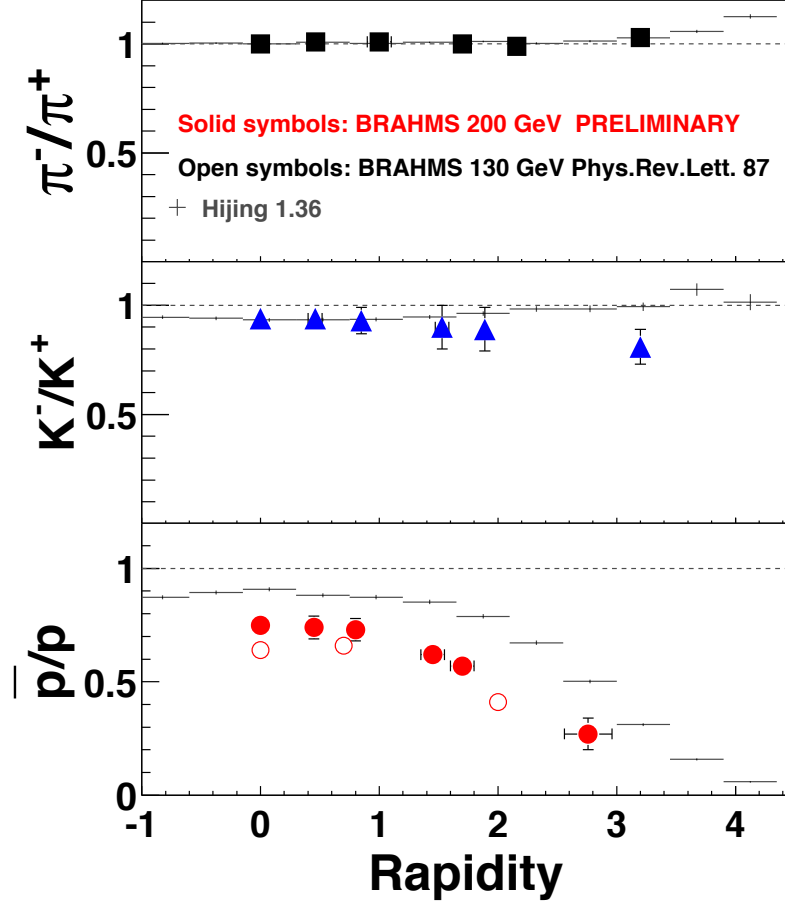
Fig. 14. Anti-particle to particle ratios as a function of rapidity for \pi^-/\pi^+ (top panel), K^-/K^+ (middle panel), \bar{p}/p (bottom panel). The crosses are the corresponding ratio predicted by HIJING model. The open symbols from the bottom refer to the data at \sqrt{s_{NN}} = 130 GeV. The horizontal errors show the rapidity interval covered, and the vertical error are the statistical only.
