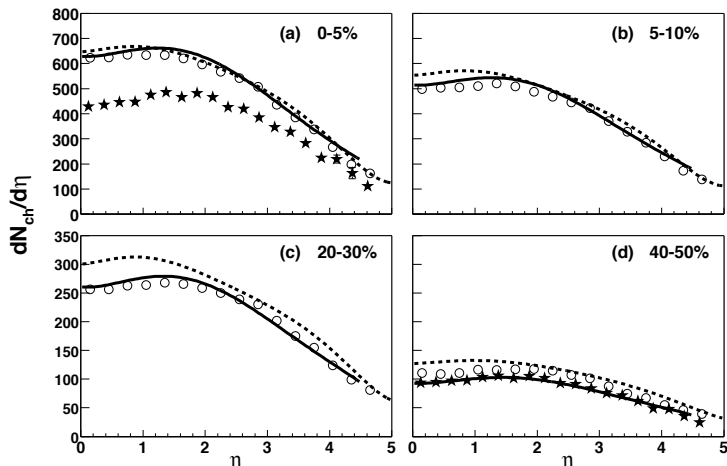
Fig. 4. (a-d) Measured dN_{ch}/d\eta distributions for centrality ranges of 0-5%, 5-10%, 20-30% and 40-50%. Theoretical predictions by Kharzeev and Levin (solid line) and by the AMPT model (dashed line) are also shown. Result from p\bar{p} collisions at \sqrt{s}=200 GeV [16], scaled by the Au+Au values of \langle N_{part} \rangle / 2 , are shown with stars (a,d).
