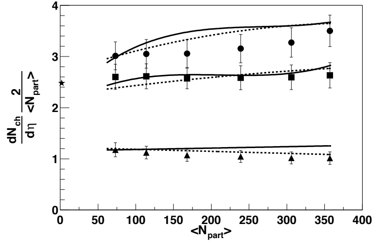
Fig. 7. dN_{ch}/d\eta per participant nucleon pair as a function of the average number of participants (see table) for \eta=0 (circles), 3.0 (squares) and 4.5 (triangles). The curves show the model predictions (see Fig. 3 caption). The star denotes the p\bar{p} result at \eta=0 [16].
