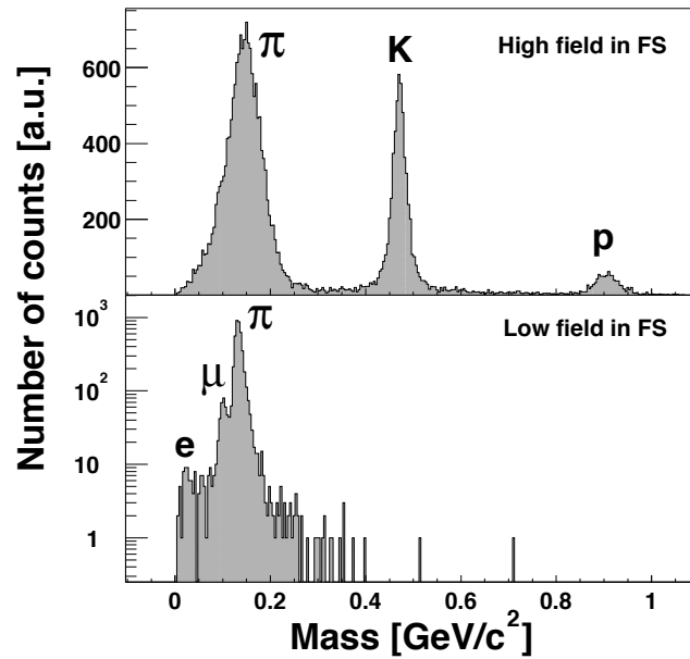
Fig. 10. Mass distribution of particles identified by the RICH detector. The low field data (bottom panel) and the high field data (top panel) particle's momenta ranging from 3 to 6 GeV/c and 8 to 20 GeV/c, respectively.
