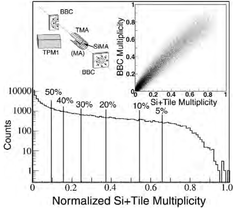
Fig. 2. Normalized MA array multiplicity distribution, as discussed in the text. The scatter plot insert shows the correlation of the normalized BBC and MA multiplicities. A schematic drawing of the global detectors used in the measurement, excluding the ZDCs, is also shown.
